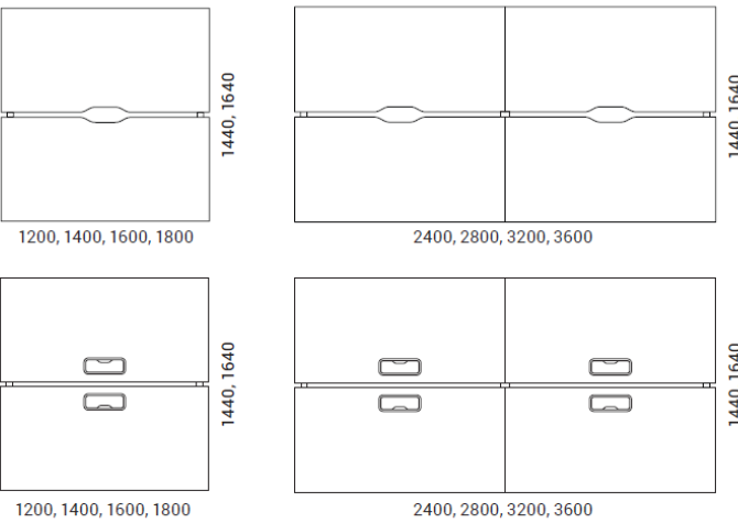
Rectangular fix
