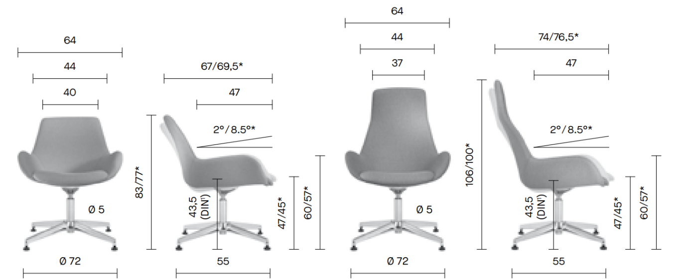
Weight: 10,7 kg
