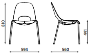
Tauko 4L-METAL weight: 5.60 kg
