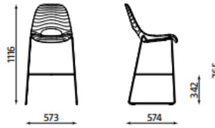
Tauko HOCKER A-PLUS CFS-ROD weight: 8.80 kg
