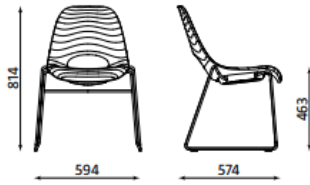
Tauko A-PLUS CFS-ROD weight: 6.60 kg
