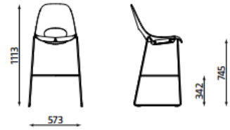
Tauko Hocker CFS-ROD weight: 8.30 kg
