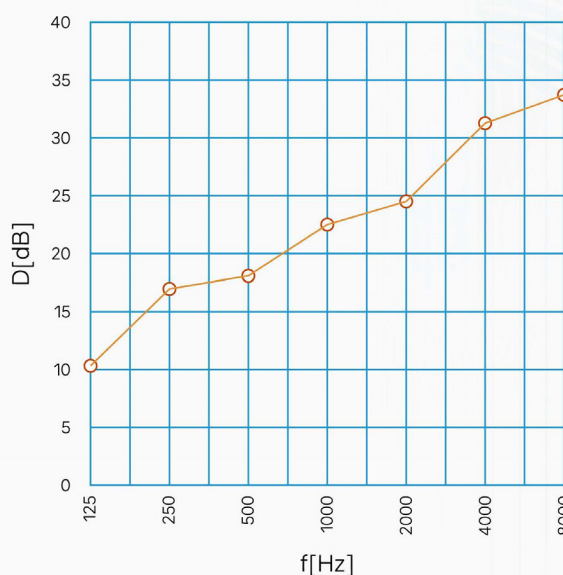
Figure 1. Speech level reduction D against 1/1 Oct Frequency
